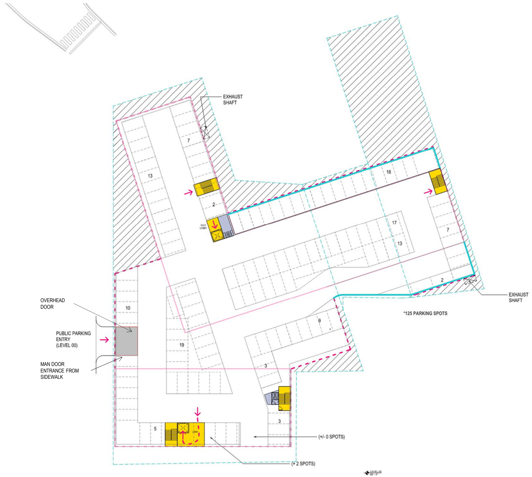
LEVEL 00
